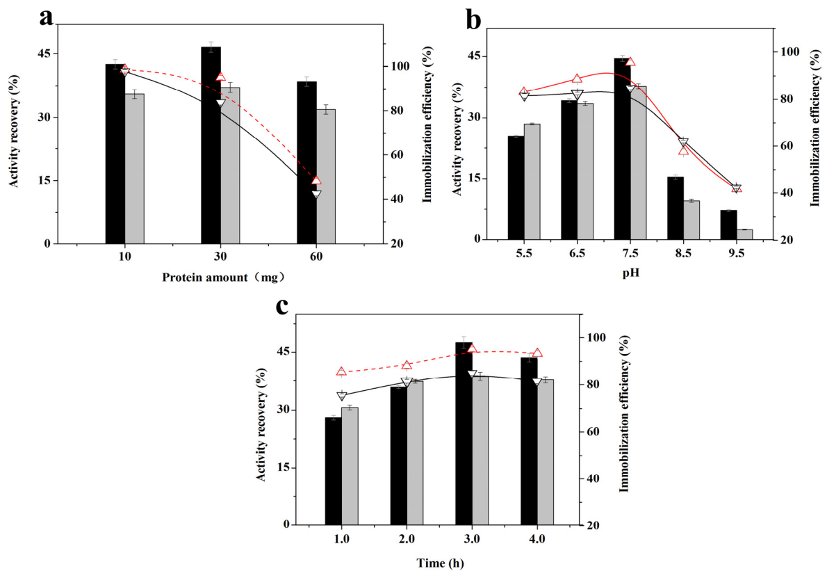
Fig. S1. Effects of enzyme amount (a), pH of Tris-HCl (b) and immobilization time (c) on the immobilization of enzymes: activity recovery of ER-FPP (■) and GDH-FPP (▒); immobilization efficiency of ER-FPP (△) and GDH-FPP (▽).
