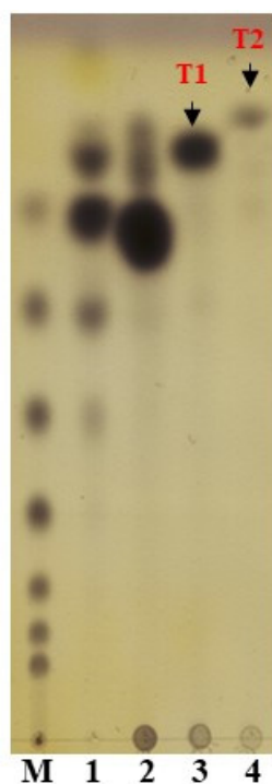
Fig. S1. TLC analysis of separated new products in Figure 1.
