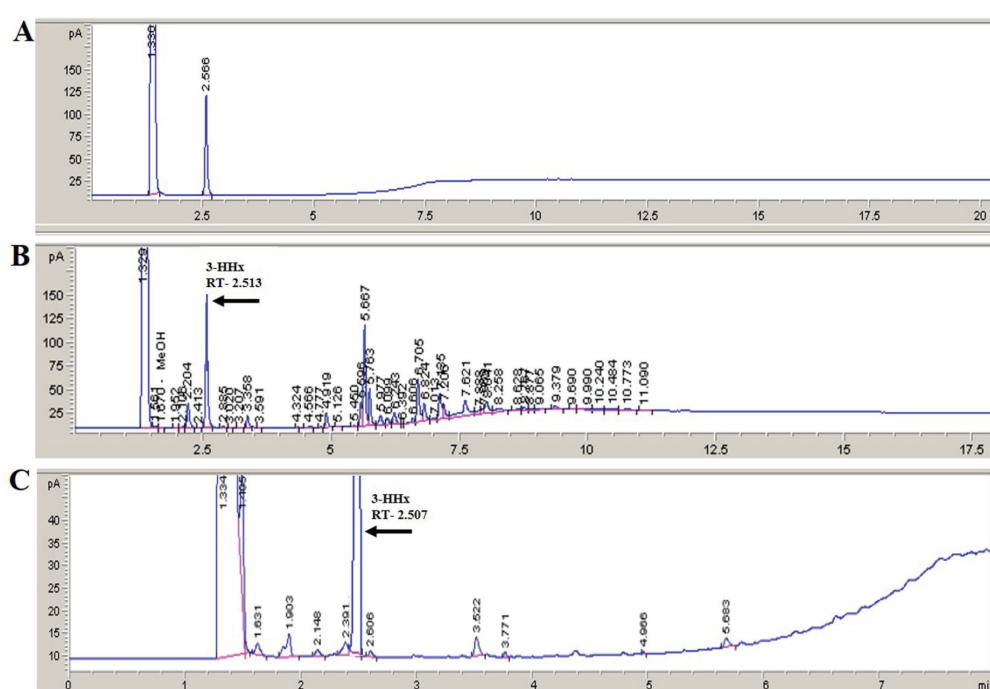
Fig. S1: GC-spectrum of 3-HHx. (A) Standard 3-HHx. (B) 3-HHx found at about same retention time (RT) with naphthalene and (C) anthracene.
