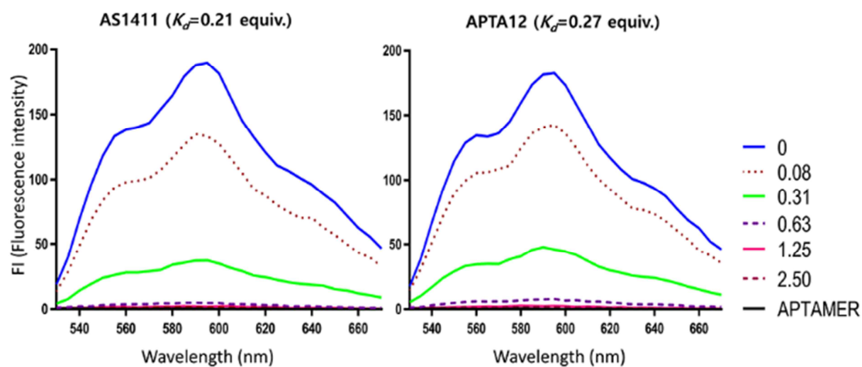
Sup. 1. Physical conjugate of APTA12 with DOX. Fluorescence spectra of doxorubicin solution (20 \mu\text{M} ) with increasing molar ratios of aptamers.
