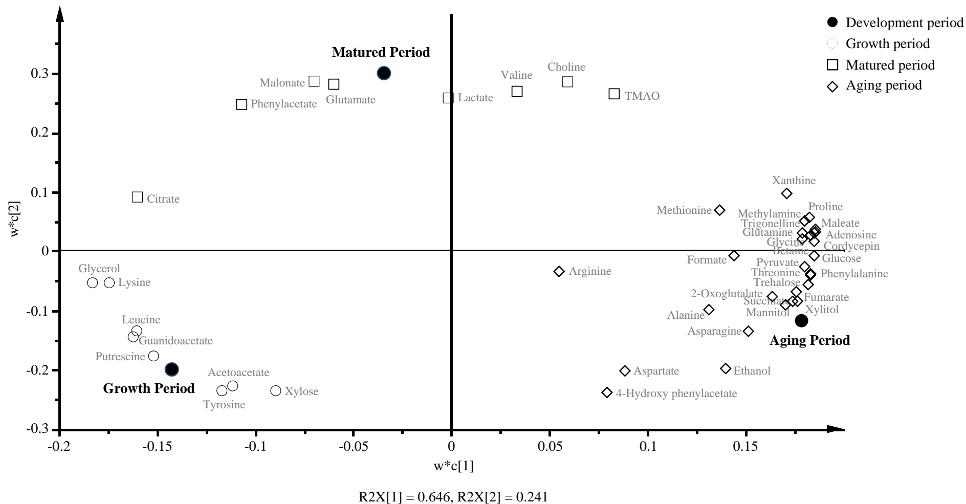
Fig. S1. Loading scatter plot for PLS-DA analysis of 50% ethanol extracts of C. militaris fruit bodies from three development periods: growth period, circular; matured period, square; aging period, diamond.
