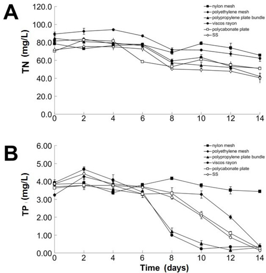
Fig. S2. Total nitrogen and phosphorus removal efficiencies of Stigeoclonium sp. HS1 in different culture systems.
