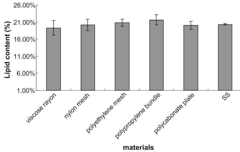
Fig. S1. Lipid content of Stigeoclonium sp. HS1 in different attached materials.
