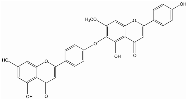
Fig. 1. Chemical structure of isocryptomerin isolated from Selaginella tamariscina .
